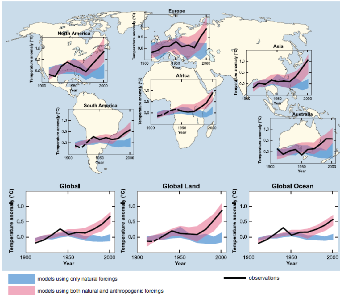
Global and continental temperature change
